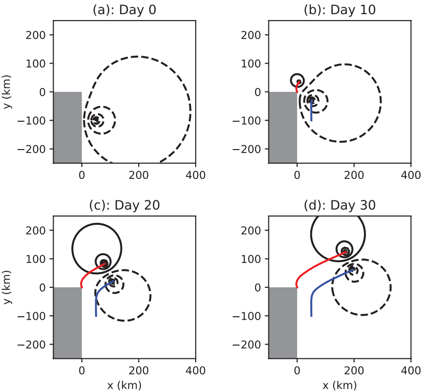
Figure 5. The blue and red lines mark the trajectory of the primary and secondary vortices, respectively. Time evolution of the stream function at (a) 0, (b) 10, (c) 20, and (d) 30 days. Dashed contours are negative values, and solid contours are positive values. Contour interval is 5.5 \times 10^3 \text{ m}^2 \text{ s}^{-1} . The x - and y -axis are in kilometers.
