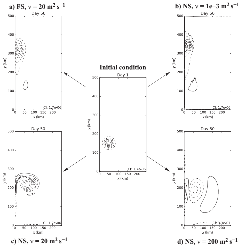
Figure 2. Different scenarios for the vortex-wall interaction: the center panel is the initial vorticity field. The other four panels are the final vorticity after 50 days with (a) free-slip (FS) boundary condition; (b) no-slip (NS), \nu = 10^{-3} \text{ m}^2 \text{ s}^{-1} ; (c) no-slip, \nu = 20 \text{ m}^2 \text{ s}^{-1} ; and (d) no-slip, \nu = 200 \text{ m}^2 \text{ s}^{-1} . The contour interval is the same for all panels except for panel (d).
